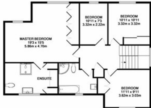
1ST FLOOR APPROX. FLOOR AREA 888 SQ. FT. (82.5 SQ. M.)
