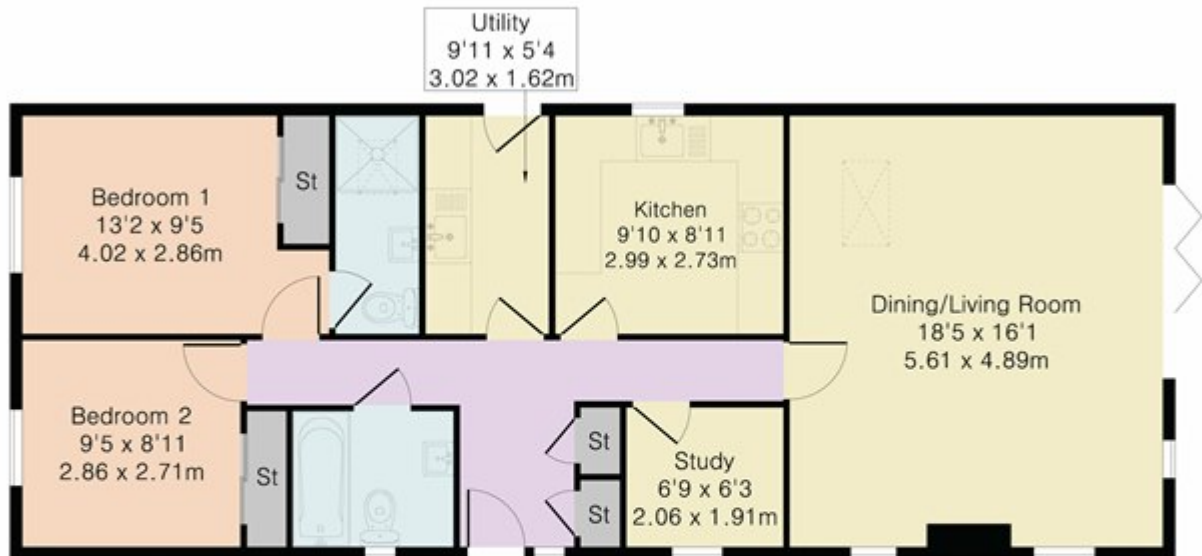
Ground Floor
